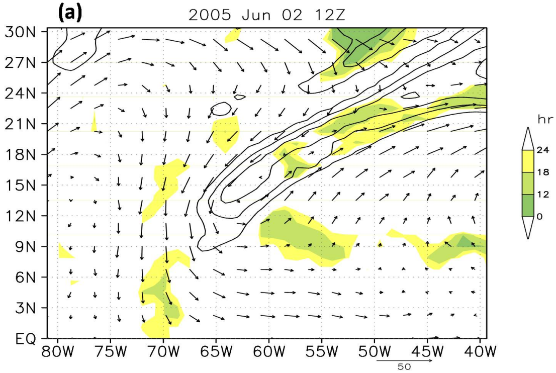
Figure 3: Filamentation time in hours (shading), potential vorticity (black contours, with a contour interval of 1 PVU starting at 2 PVU), and wind vectors in \text{m s}^{-1} on the 360 K isentropic surface for (a) 2 June 2005 12 UTC, (b) 3 June 2005 00 UTC, (c) 3 June 2005 12 UTC, (d) 4 June 2005 00 UTC, (e) 4 June 2005 12 UTC. In the unshaded areas, the flow is either vorticity dominated or has a filamentation time that is negative or longer than 24 hours. The scale for the wind vectors ( 50 \text{ m s}^{-1} ) is given at the bottom of the figure.
