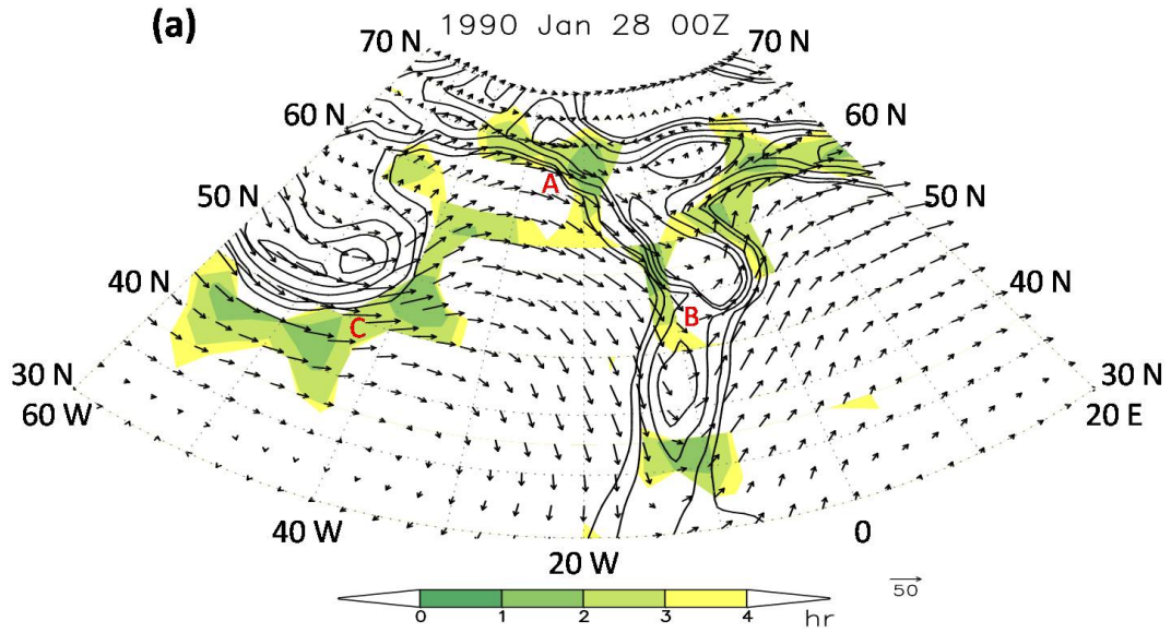
Figure 1: Filamentation time in hours (shading), potential vorticity (black contours, with 1, 2, 4, 6, 8 PVU), where PVU stands for a “PV unit” of 10^{-6} \text{ m}^2 \text{ s}^{-1} \text{ K kg}^{-1} , and wind vectors in \text{m s}^{-1} on the 310 K isentropic surface for (a) 28 Jan 1990 00 UTC, (b) 28 Jan 1990 12 UTC, (c) 29 Jan 1990 00 UTC, (d) 29 Jan 1990 12 UTC. In the unshaded areas, the flow is either vorticity dominated or has a filamentation time that is negative or longer than 4 hours. The scale for the wind vectors ( 50 \text{ m s}^{-1} ) is given at the bottom of the figure.
