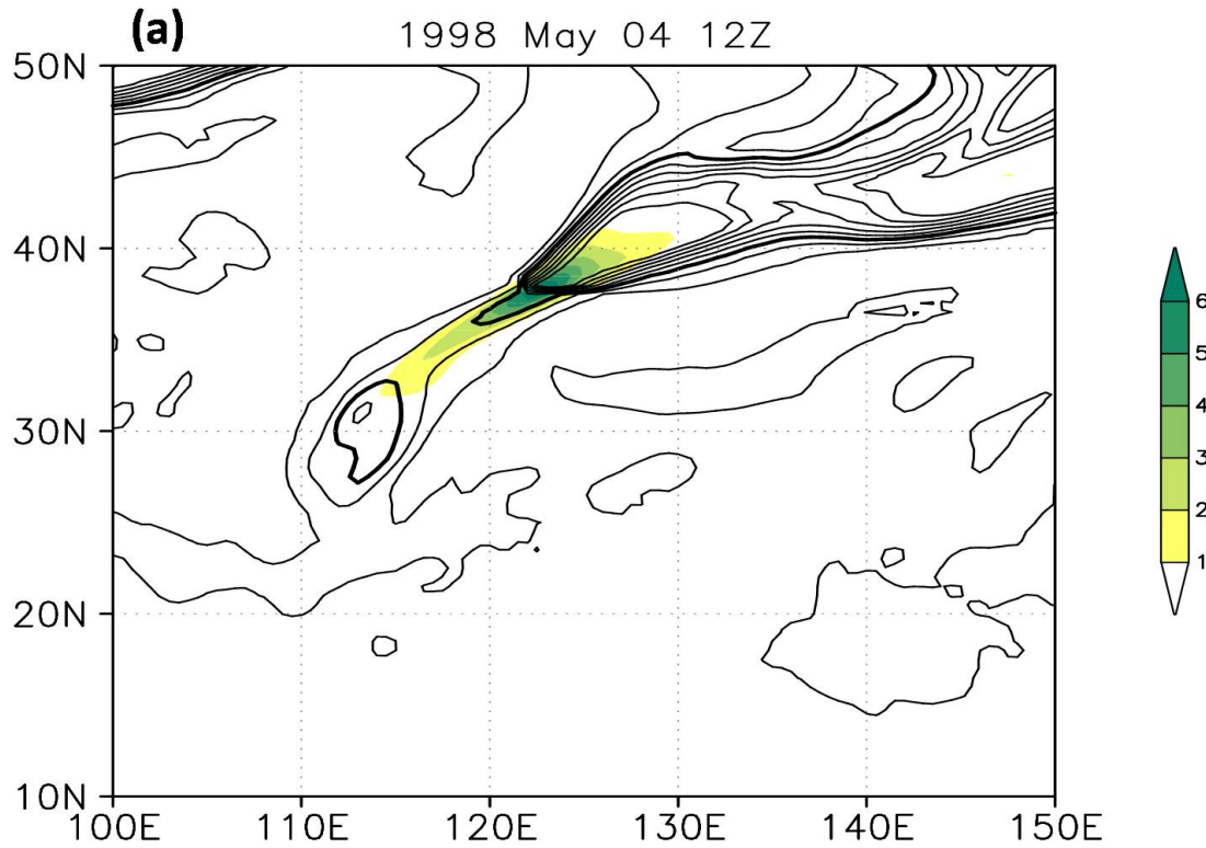
Figure 5: The potential vorticity (black contours, in PVU), and the deformation field (shading): (a) square of the stretching deformation in 10^{-8} \text{ s}^{-2} for 4 May 1998 12 UTC; (b) square of the stretching deformation in 10^{-9} \text{ s}^{-2} for 3 June 2005 12 UTC; (c) square of the shearing deformation in 10^{-9} \text{ s}^{-2} for 3 June 2005 12 UTC. We only analyse the filamentation zone in the trough for the TUTT case.
