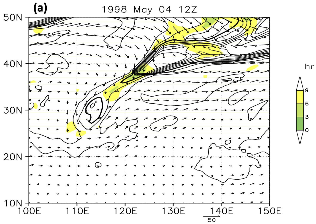
Figure 4: (a) The same as Fig. 2b but without the divergence term. (b) The same as Fig. 3c but without the divergence term.
