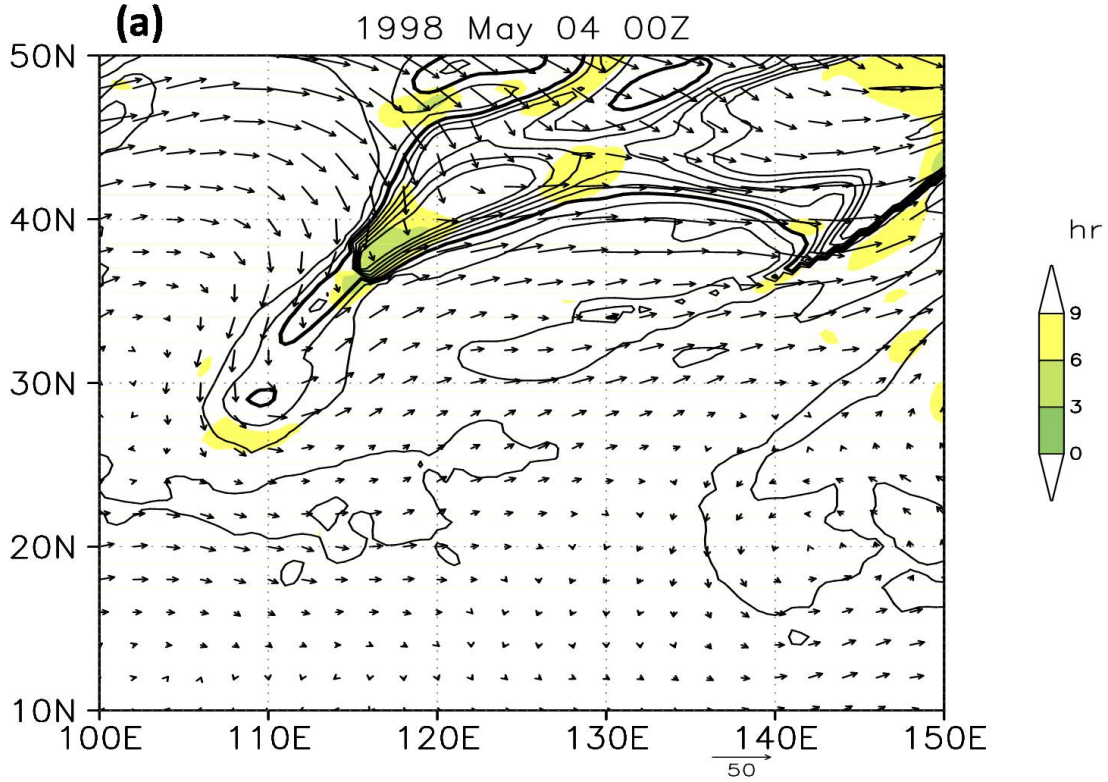
Figure 2: Filamentation time in hours (shading), potential vorticity (black contours, with a contour interval of 0.5 PVU starting at 0.5 PVU), and wind vectors in \text{m s}^{-1} on the 330 K isentropic surface for (a) 4 May 1998 00 UTC, (b) 4 May 1998 12 UTC, (c) 5 May 1998 00 UTC, (d) 5 May 1998 12 UTC. In the unshaded areas, the flow is either vorticity dominated or has a filamentation time that is negative or longer than 9 hours. The bold solid line is the 1.5 PVU contour, which represents the dynamic tropopause. The scale for the wind vectors ( 50 \text{ m s}^{-1} ) is given at the bottom of the figure.
